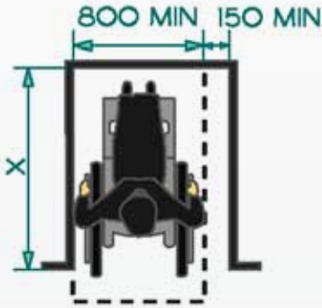
FRONTAL APPROACH - WHERE X IS MORE THAN 610
