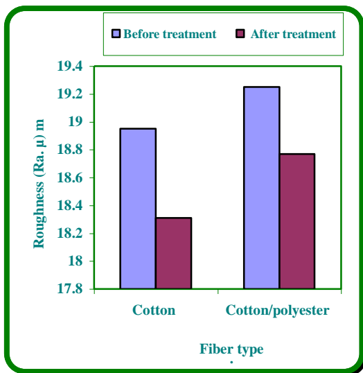
Fig .(11 ) Effect of fiber type on roughness after and before treatment , at blend samples and 27 picks/cm and twill 2/2.
