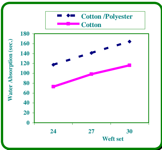
Fig .(13 ) Effect of fiber type and weft set after treatment ,at satin 4
