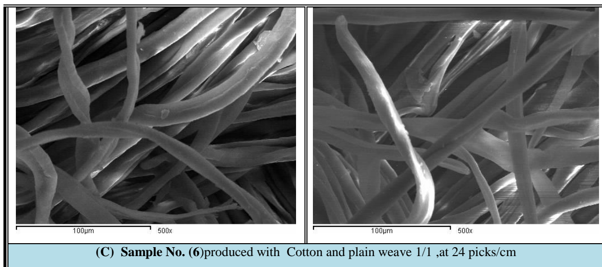
Fig. (2) Scanning electron micrograph (SEM) of different cotton fabrics before and after treatment .
