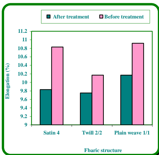
Fig.(7) effect of fabric structure on elongation, at 27 picks/cm and cotton samples, after and before treatment
