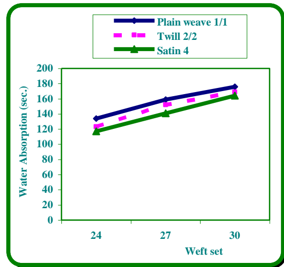
Fig .(14 ) Effect of weft set and fabric structure on water absorption after treatment , at 50/50 cotton/polyester blend samples.
