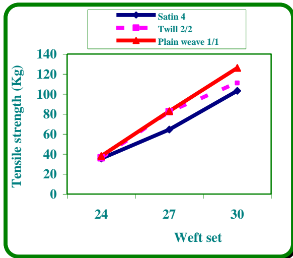
Fig.(5) effect of weft set and fabric structure on tensile strength, at 50/50 cotton/polyester blend samples, after treatment
