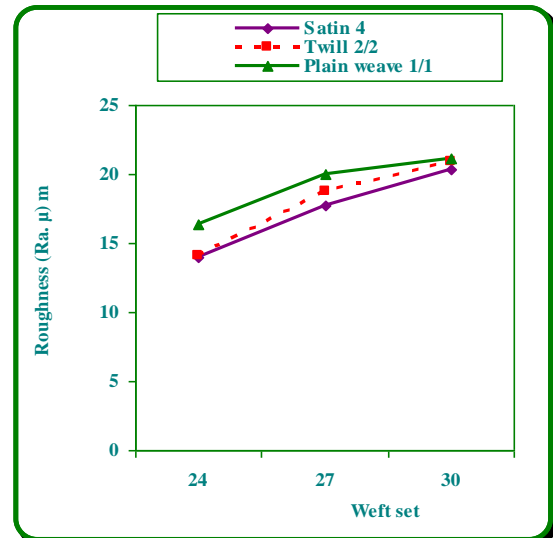
Fig .( 12) Effect of weft set and fabric structure on roughness after treatment, at 50/50 cotton/polyester blend samples
