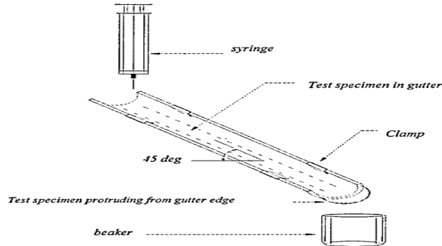
FIGURE 1. Gutter test apparatus.
